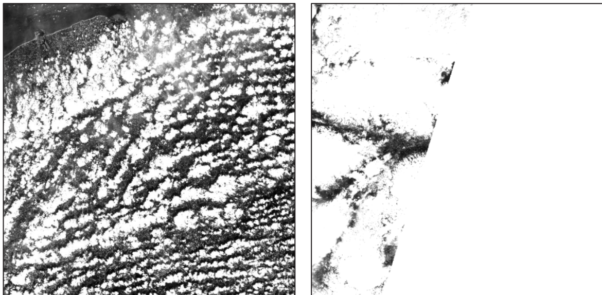
Figure 6.2 Quicklooks of tile 31UES S2A acquired on (left) 24-08-2017 and (right) 06-09-2017.
