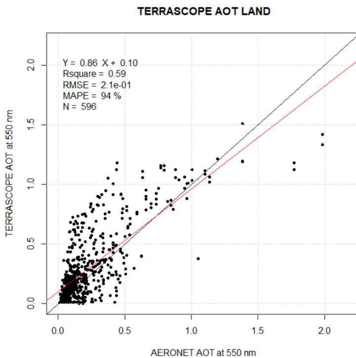
Figure 6.11 Terrascope AOT validation LAND
