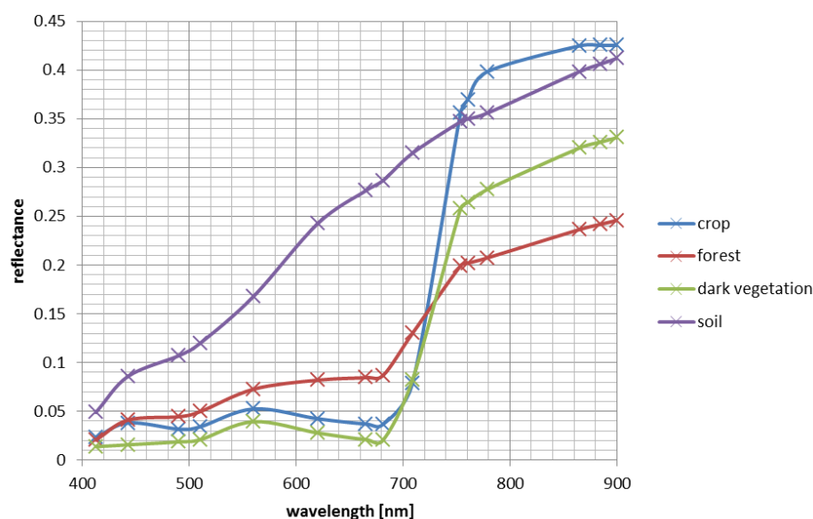
Figure 2.4 Spectral reflectance of the four endmembers used in the iCOR land-based AOT retrieval
