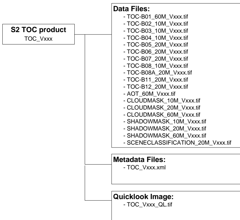
Figure 3.1: S2 TOC product file list
