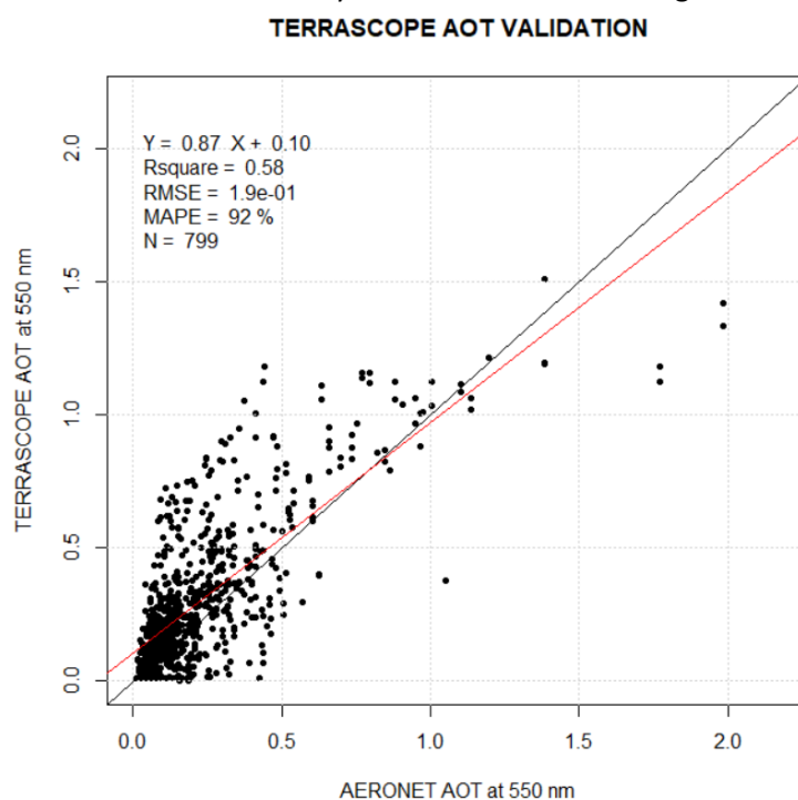
Figure 6.9 Terrascope AOT validation
