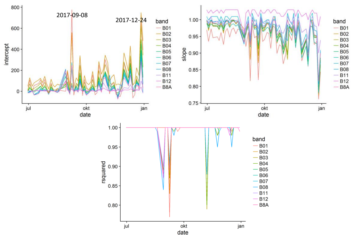
Figure 6.3 Regression statistics between TOC products of V101 and V102 for 31UES – Sentinel-2B tiles. (top left) intercept (*10000) (top right) slope and (bottom) the coefficient of determination ( R^2 ) values for the different S2A spectral bands.
