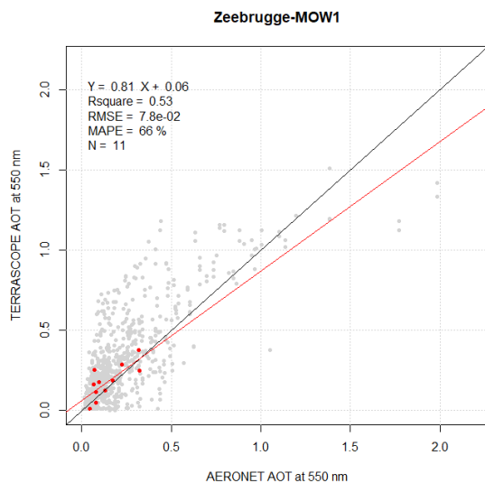
Figure 6.12 Scatterplots of AOT at 550 nm used in the Terrascope chain compared to AERONET measurements for individual sites. The red dots represent the values for each specific site, while the grey dots are all match-ups.
