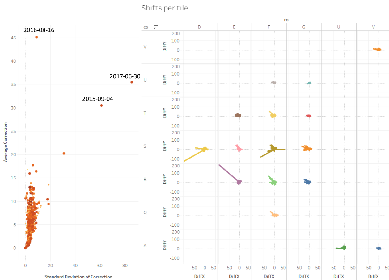
Figure 6.4 Geometric shifts of the S2 data. (l) The final shift parameter, expressed in meter, applied for each tile and the corresponding standard deviation noted within one tile. (r) Detention into the Individual shift parameters noted for each shapefile, expressed in meter for the two spatial dimensions.
