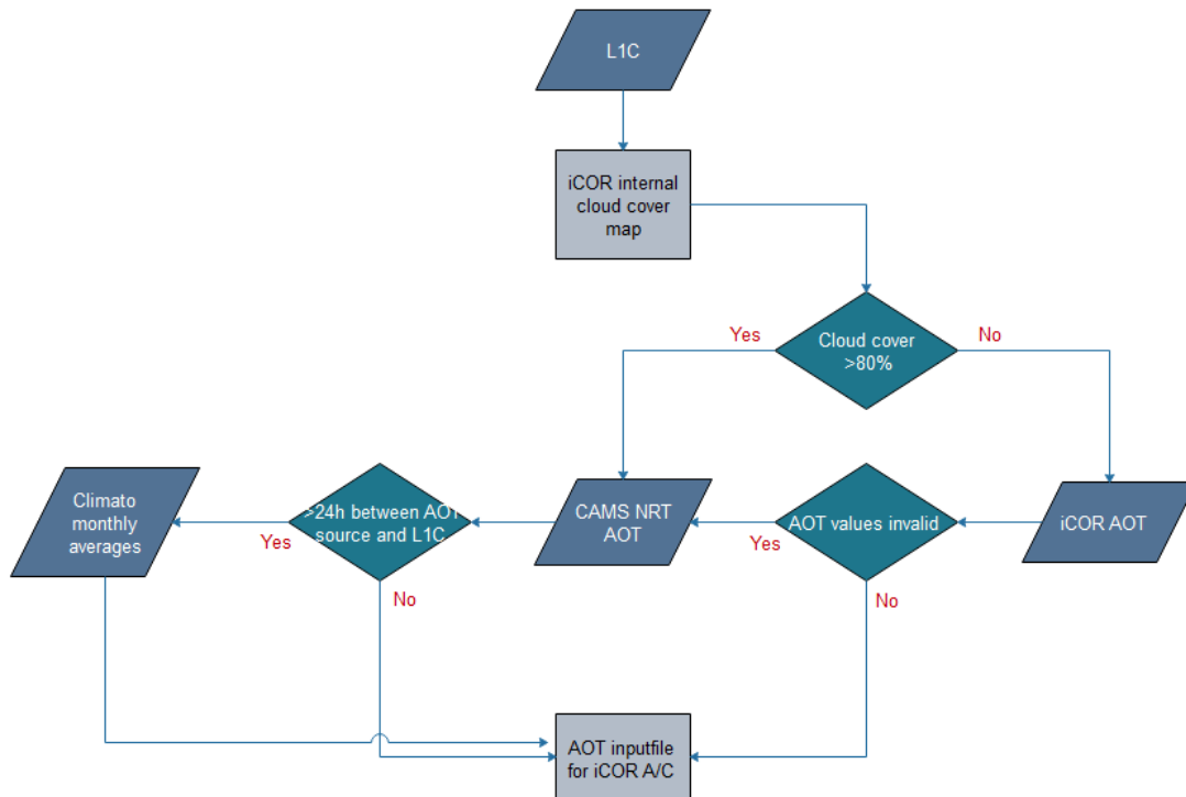
Figure 4.3: Flowchart explaining the AOT origin
