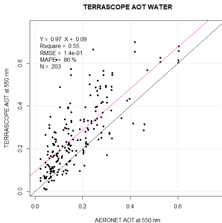
Figure 6.10 Terrascope AOT validation WATER
