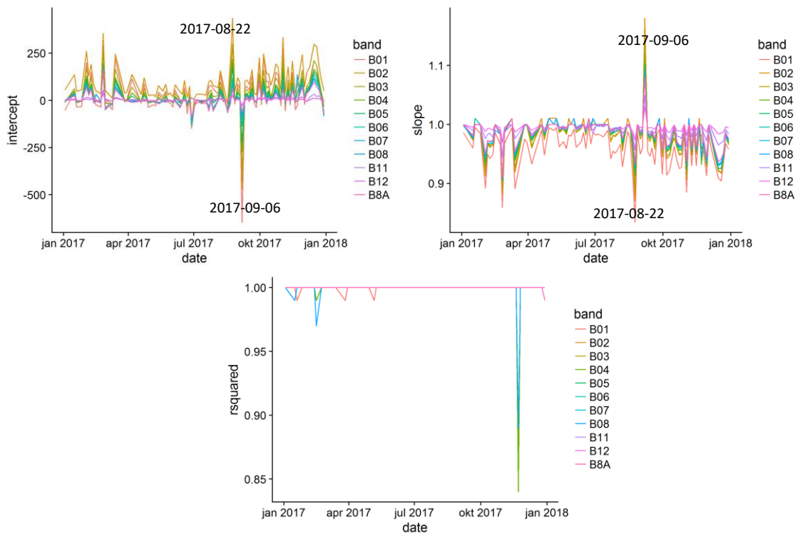
Figure 6.1 Regression statistics between TOC products of V101 and V102 for 31UES – Sentinel-2A tiles. (top left) intercept (*10,000) (top right) slope and (bottom) the coefficient of determination ( R^2 ) values for the different S2A spectral bands.
